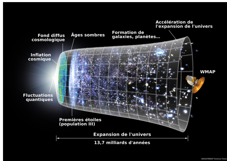
FIGURE 5 – Expansion de l'Univers
