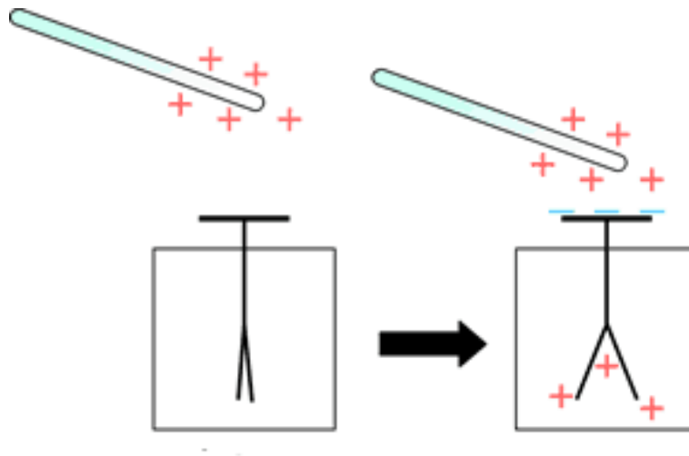
FIGURE 1 – Electroscopie
